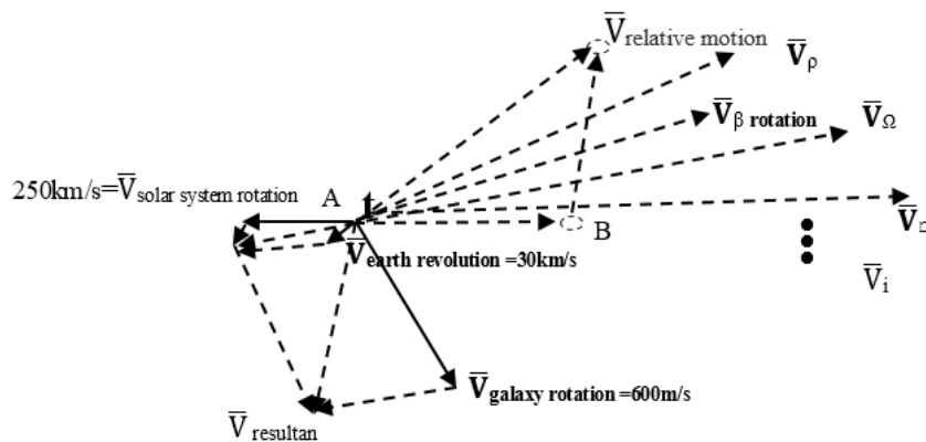
FIG.2. Examples of velocity relative to the earth's universe at all levels.
