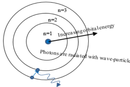
FIG.8. Electron migration releases photons.
