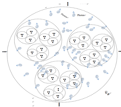
FIG.7. \rho World level many of \beta world (level) compose \rho world (level).
