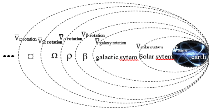
FIG.1. Matter Hierarchy Map in the Universe [2-3].
