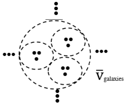
FIG.5. Planet World and galaxies compose Similar river system(level).
