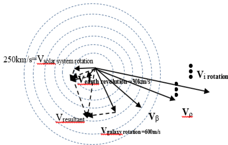
FIG.3. Multi layer Matter motion direction relation diagram.
