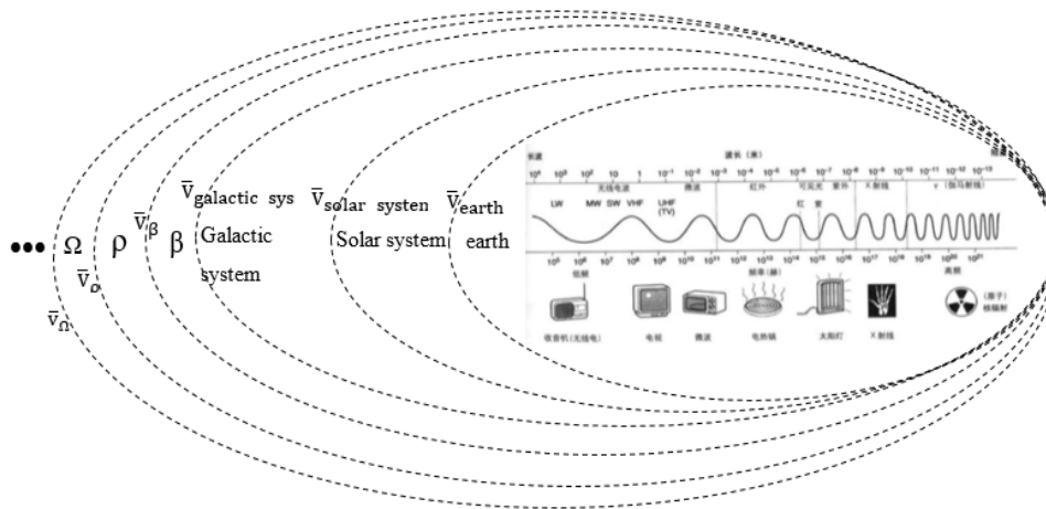
FIG.10. Formation of the Electronic waveform.
