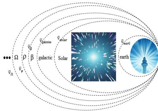
FIG.9. Schematic diagram of photon motion.
