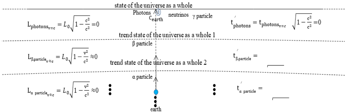
FIG.11. Trajectory diagram of particle motion.
