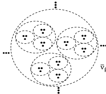
FIG.5. Planet World and galaxies compose Similar river system(level).
