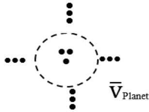
FIG.4. Planet World level Many atoms made up Planet World(level).
