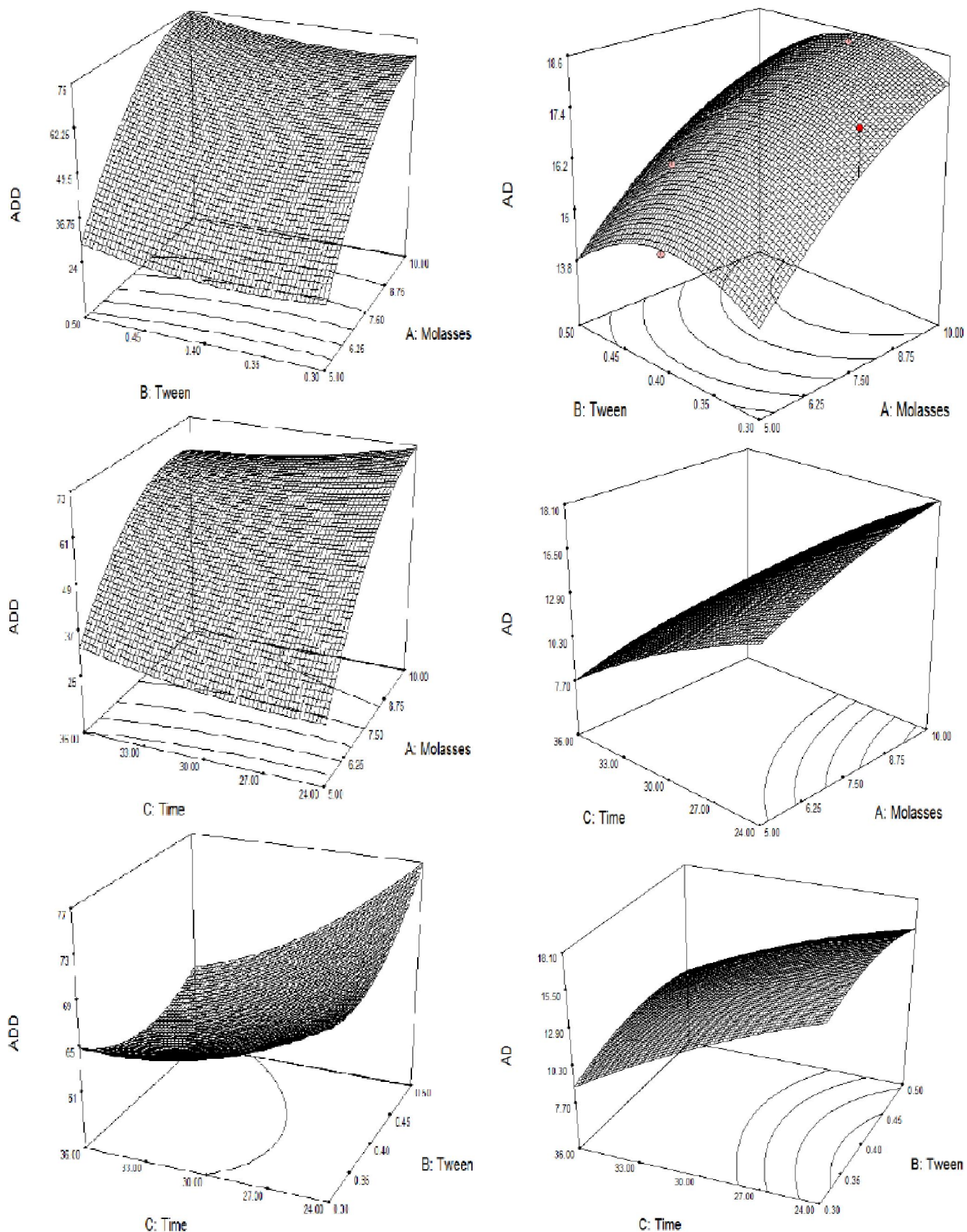
Figure 8 : The interaction between the most significant factors affection the conversion of sterols to AD and AADD according to Box-Behnken model
