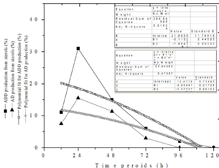
Figure 3 : The optimum time for the conversion of the sterols to AD and ADD
