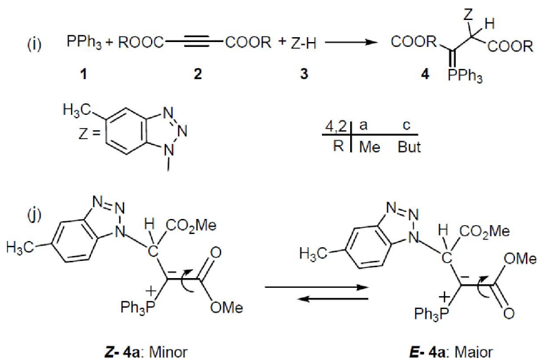
Figure 1 : (i) The reaction between triphenylphosphine 1, dialkyl acetylenedicarboxylate 2 (2a or 2c) and 5-methyl Benzotriazole 3 for generation of stable phosphorus ylides 4 (4a or 4c). (j) The two isomers Z -4a and E -4a (minor and major, respectively) of ylide 4a
