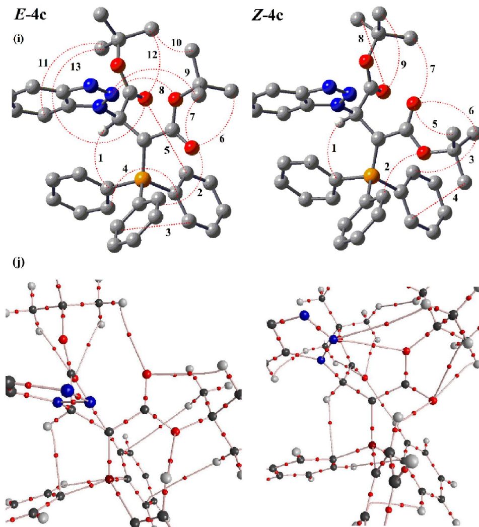
Figure 3 : (i) Intramolecular hydrogen bonds (dotted lines) in the two E-4c and Z-4c geometrical isomers of stable ylide 4c, (j) Part of molecular graphs, including intramolecular hydrogen bond critical points (BCPS) for the two rotational isomers such as E-4c and Z-4c . Small red spheres, and lines corresponding to BCPS bond paths, respectively
