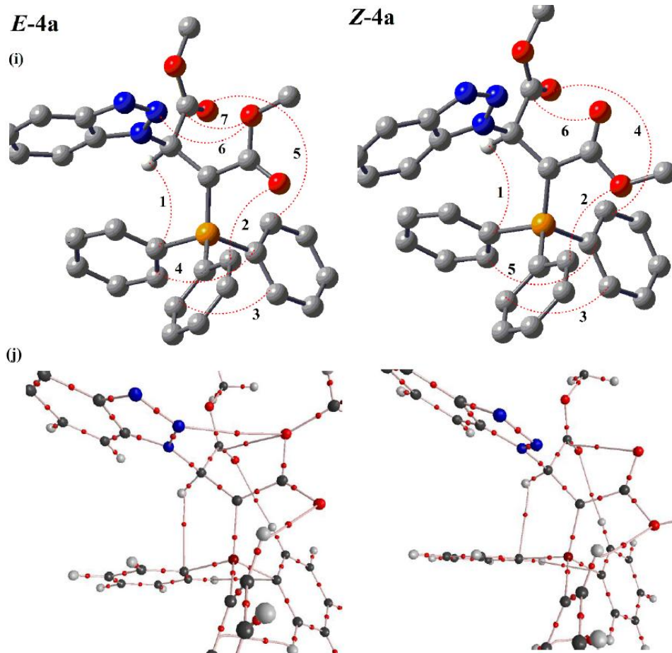
Figure 2 : (i) Intramolecular hydrogen bonds (dotted lines) in the two E -4a and Z -4a geometrical isomers of stable ylide 4a, (j) Part of molecular graphs, including intramolecular hydrogen bond critical points (BCPS) for the two rotational isomers such as E -4a and Z -4a. Small red spheres, and lines corresponding to BCPS bond paths, respectively
