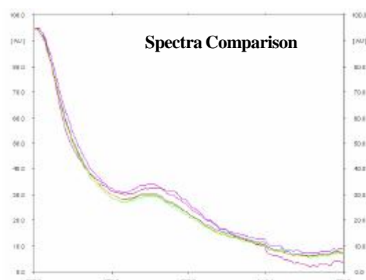
Figure 8: Overlay spectra of spectra of withanolide precision
