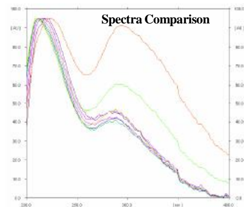
Figure 9: Overlay spectra of shatavarin at concentration 4-12 \mu g
