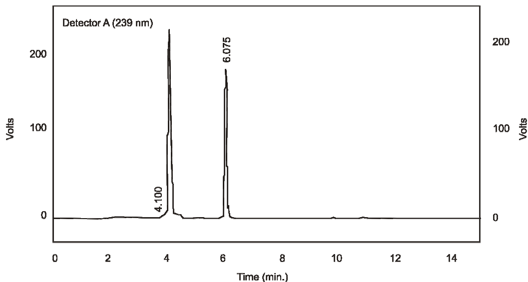
Fig. 2: A typical chromatogram of simvastatin and ezetimibe reference substance
