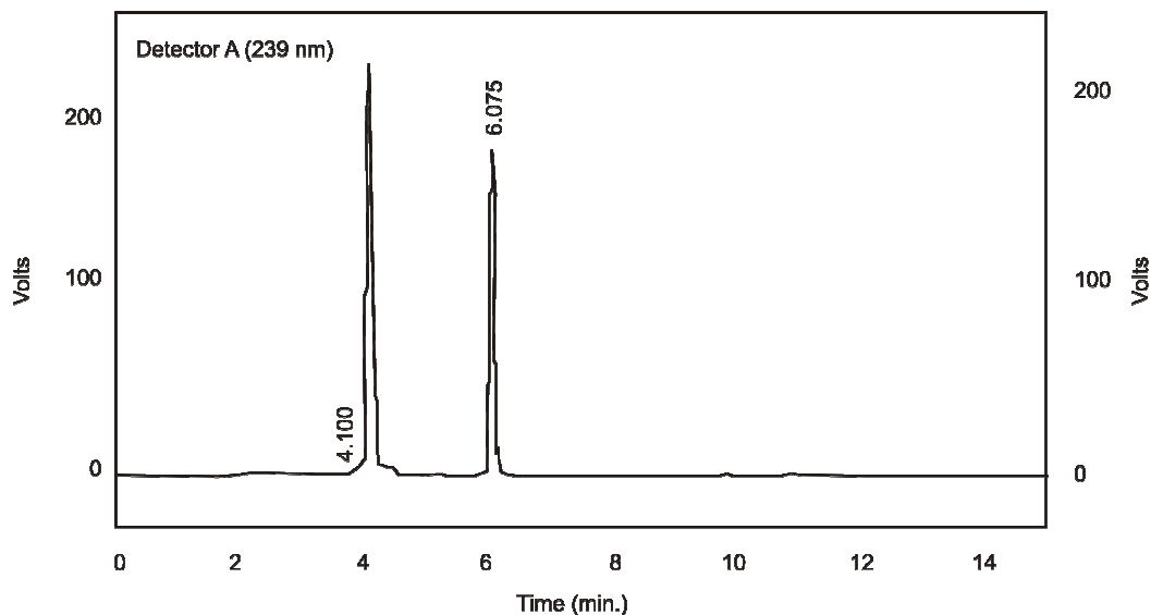
Fig. 3: A typical chromatogram of simvastatin and ezetimibe tablets
