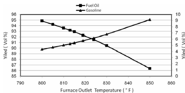
Figure 6 : Comparison of fuel oil and gasoline yield versus furnace outlet temperature
