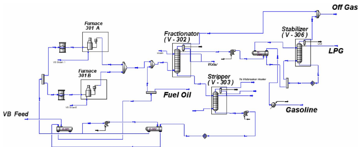
Figure 2 : Simulation of visbreaking unit at Tehran refinery
