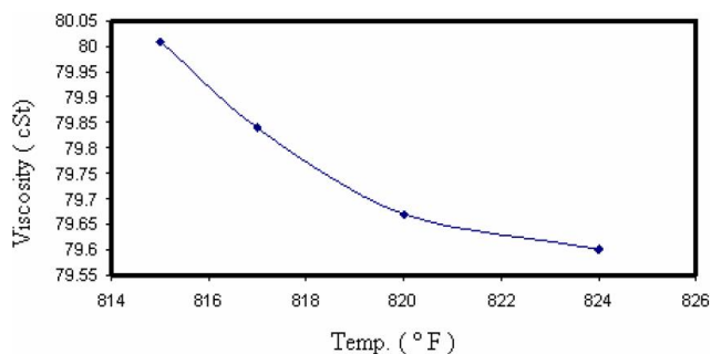
Figure 5 : Sensitivity of fuel oil viscosity versus the furnace outlet temperature
