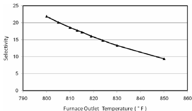
Figure7 : Selectivity of fuel oil to gasoline versus furnace outlet temperature
