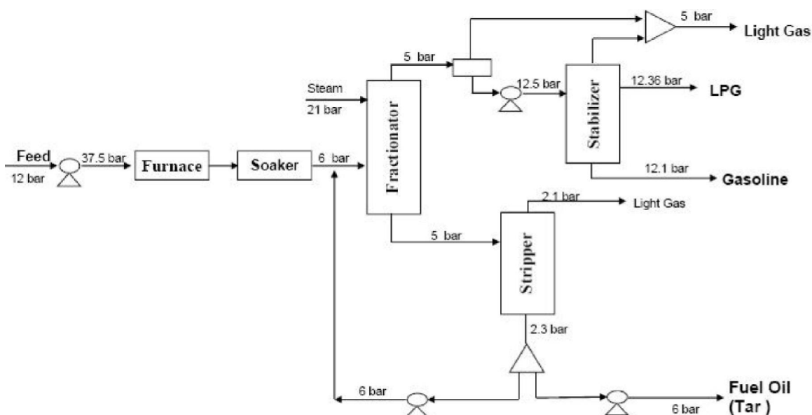
Figure 1 : Block flow diagram of visbreaking process
