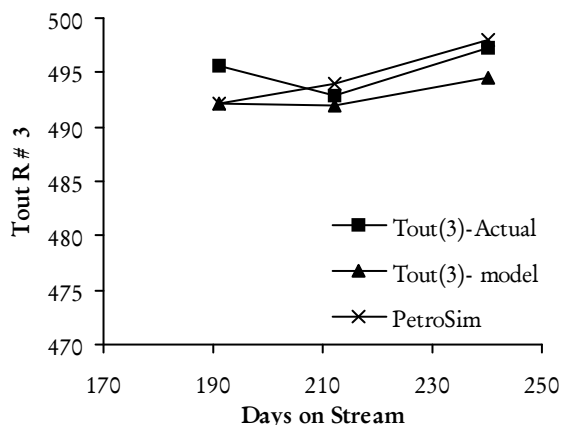
Figure 5: Comparison of outlet temperature (°C) in the third reactor
