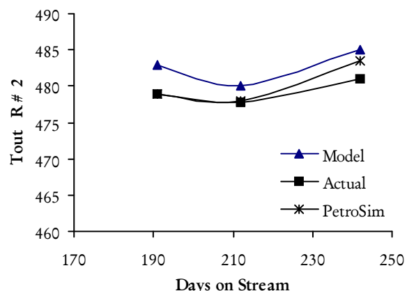
Figure 4: Comparison of outlet temperature (°C) in the second reactor
