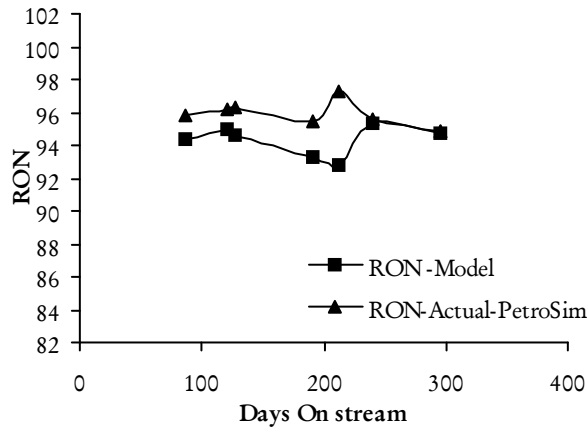
Figure 7: Comparison of RON product
