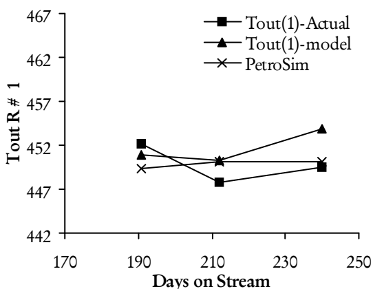
Figure 3: Comparison of outlet temperature (°C) in the first reactor
