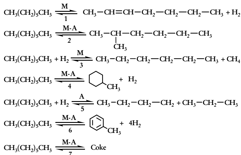
Figure 1: A typical of reactions in the catalytic reforming process
