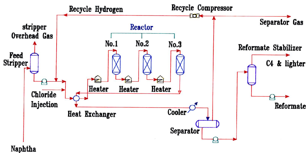
Figure 2: Catalytic reforming flowchart (semi-regenerative)
