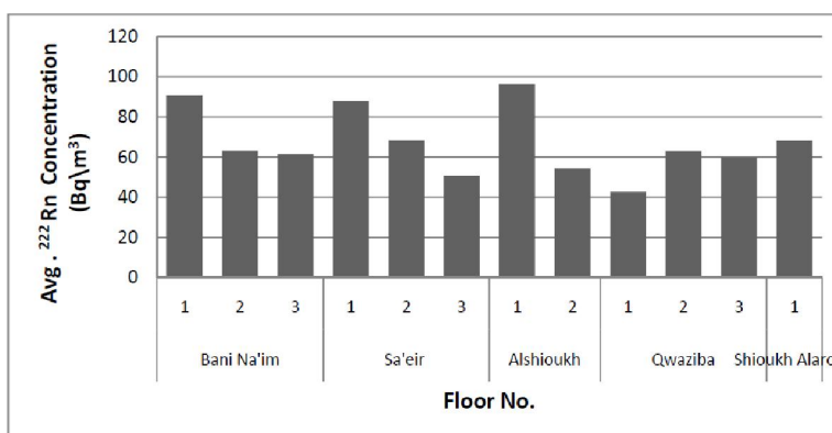
Figure 3 : Histogram showing the average radon concentration levels in different floors of the studied regions
