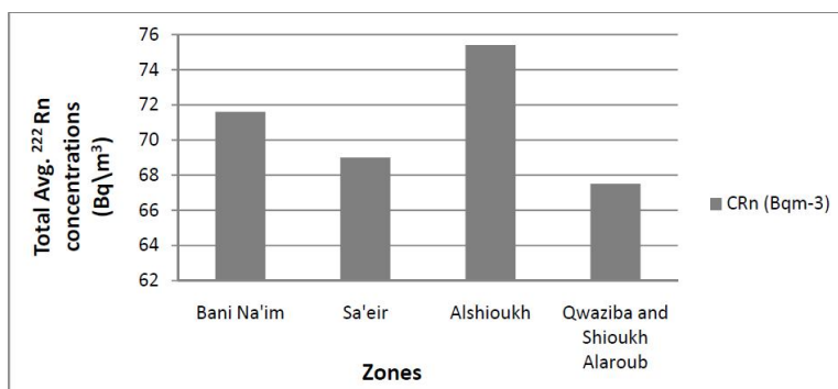
Figure 4 : The total average radon concentrations level in the different schools the studied regions
