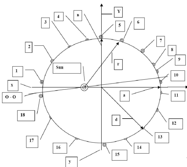
Figure 4 : Orbit of Mercury
