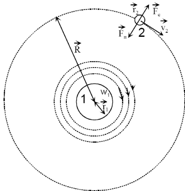
Figure 1 : Two-dimensional model of gravitational interaction of two bodies. The forces are shown acting on body 2: F_c - the centrifugal force, F_{\text{a}} - the force of attraction of body 2 from body 1; v_2 - linear velocity of body 2 at the orbit, R - the radius of the orbit, r_1 - the radius of body 1, r_2 - the radius of body 2, w_1 - angular velocity of ether rotation at the surface of body 1, and m_2 are the mass of body 2.
