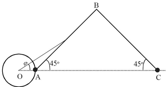
Figure 6 : Scheme of space flight; O - centre of Earth; A - start of flight; C - Moon (finish); AC - projection of gravitational flat
