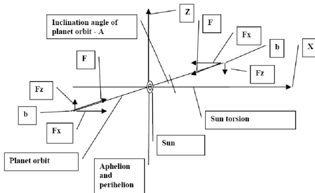
Figure 3 : Kinematical scheme of orbital motion
