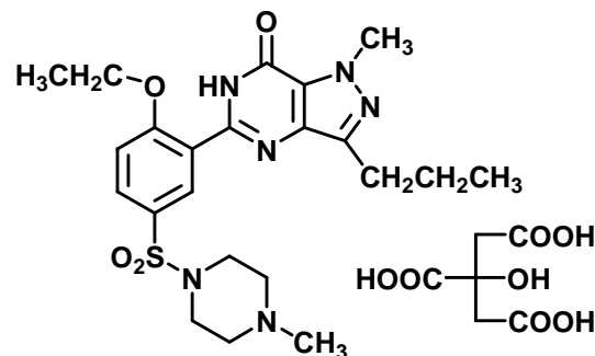
Figure 1 : Chemical structure of Sildenafil citrate
