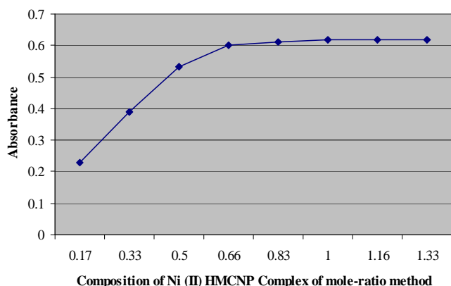
Figure 4 : Result of Yoe and Jones mole ratio method
