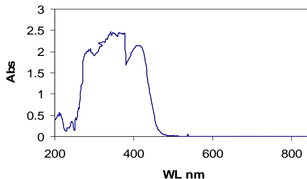
Figure 1 : Absorption spectra of Ni(II)-HMCPP complex
