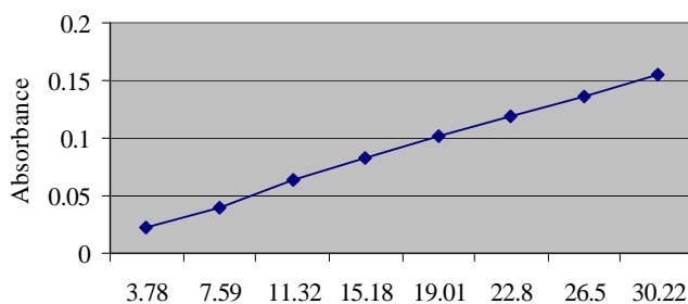
Figure 2 : Verification of Beer's law
