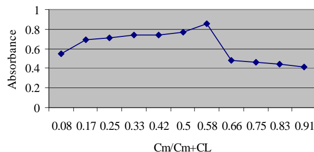
Figure 3 : Result of Job's method of continuous verification
