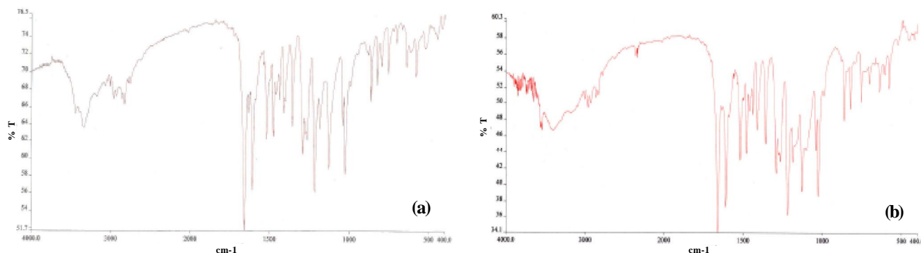
Figure 3 : IR spectrum of (a) Cu (2TMBAMP) 2 and (b) Co (2TMBAMP) 2 complex.
