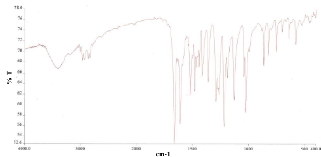
Figure 2 : IR spectrum of 2TMBAMP ligand.
