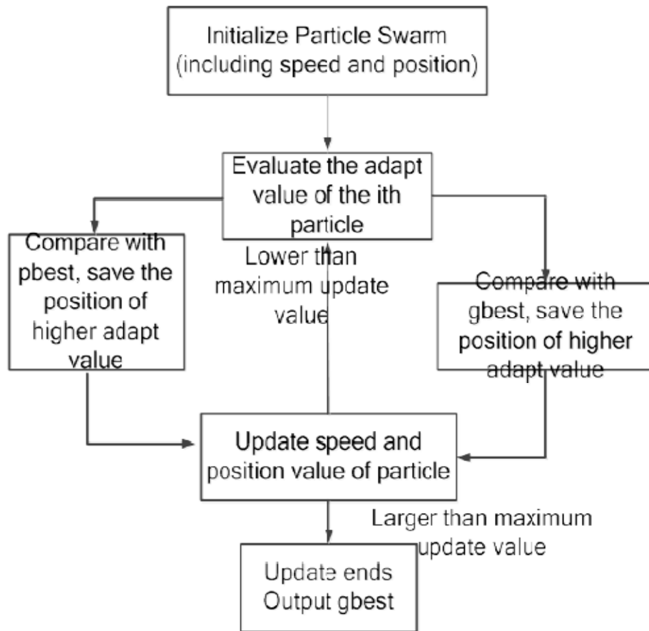
Figure 4: The standard particle swarm optimization algorithm flow chart
