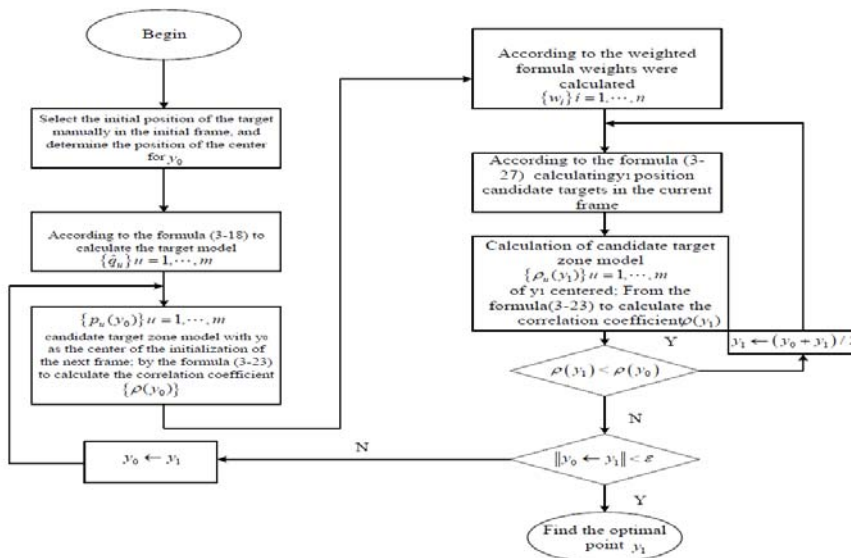
Figure 6: Mean Shift target tracking algorithm complete process
