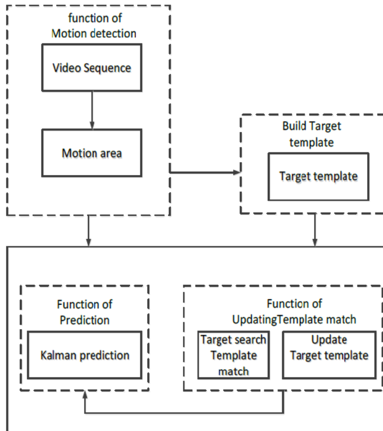
Figure 7: Target tracking algorithm flow
