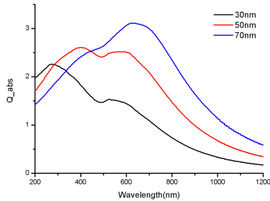
FIG. 2. Absorption spectra with different size of Au 50 Fe 50 bimetallic alloy nanoparticles.
