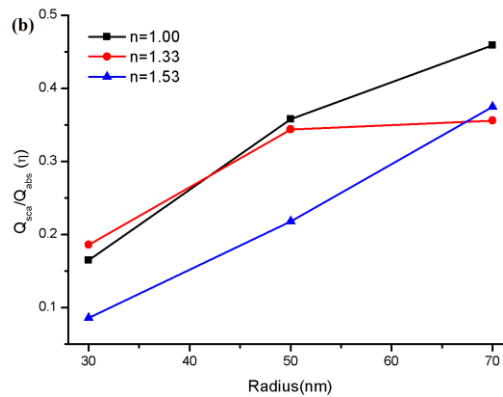
FIG. 5. Dependencies of relative efficiency on the size and medium.
