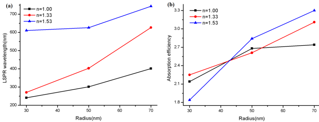
FIG. 3. (a) Effect of the medium refractive index on LSPR wavelength (b) absorption efficiency as a function of particles size.
