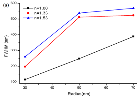
FIG. 4. Effect of the medium refractive index on FWHM of Au-Fe nanoparticles.
